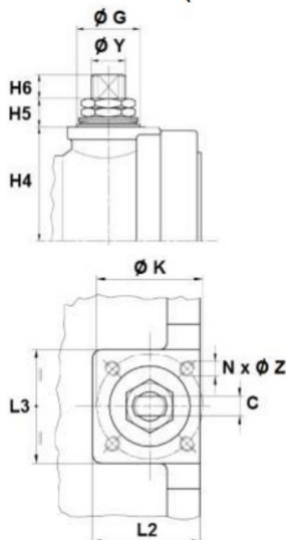
REF. 770 DN 150-200 ( TYPE FB2 )
