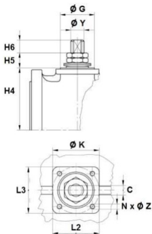
REF. 770 DN125 TYPE FB1
