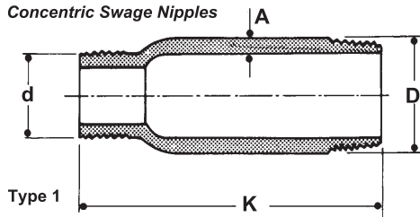
Concentric Swage Nipples
