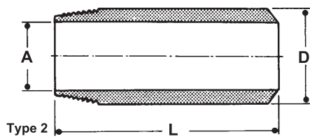
Pipe Nipple TOE
