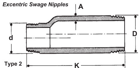
Excentric Swage Nipples
