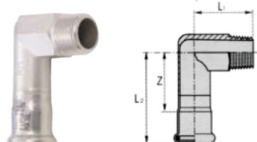
INOX PRESS - 90° Elbow F (press) / male thread BSP
