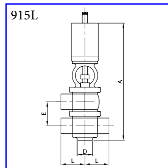
Pneumatic valve 3-A 4-ways LT - plain ends AISI 304L, AISI 316L
