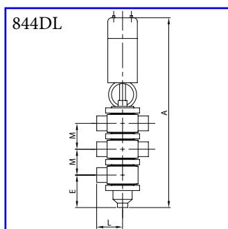
Drainage pneumatic valve 5-ways TTL - plain ends AISI 316L
