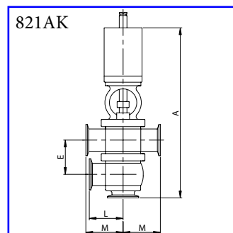
Pneumatic valve 3-A 4-ways TL - CLAMP AISI 316L
