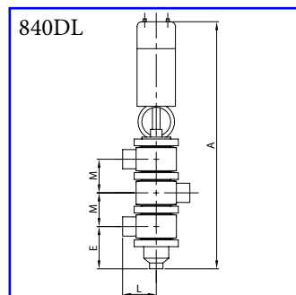
Drainage pneumatic valve 3-ways LLL - plain ends AISI 316L
