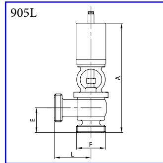
Pneumatic valve 3-A 2-ways L - male ends AISI 304L, AISI 316L
