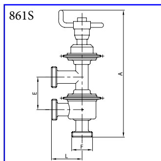
Manual valve 3-ways LL - male ends AISI 304L, AISI 316L
