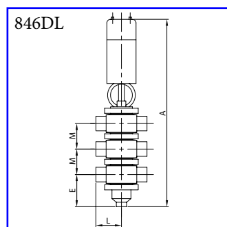
Drainage pneumatic valve 6-ways TTT - plain ends AISI 316L
