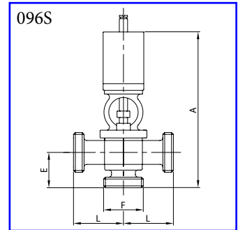
Pneumatic valve 3-A 3-ways T - male ends AISI 304L, AISI 316L
