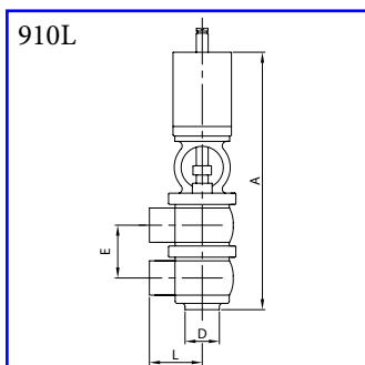
Pneumatic valve 3-A 3-ways LL - plain ends AISI 304L, AISI 316L
