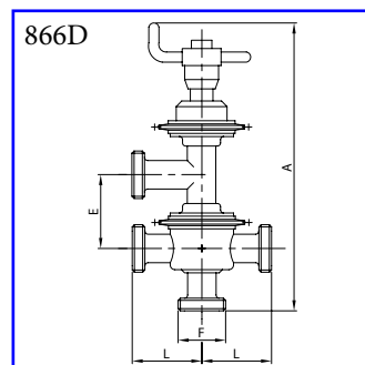
Manual valve 4-ways LT - male ends AISI 304L, AISI 316L
