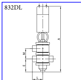
Drainage pneumatic valve 3-ways LT - plain ends AISI 316L
