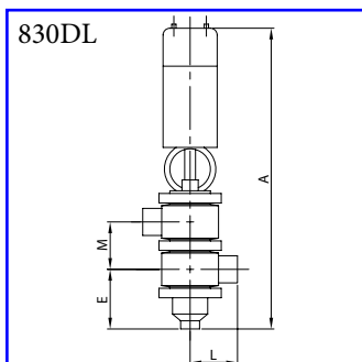
Drainage pneumatic valve 2-ways LL - plain ends AISI 316L
