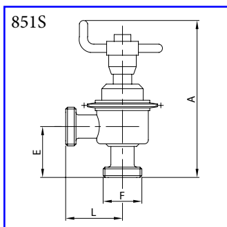
Manual valve 2-ways L - male ends AISI 304L, AISI 316L
