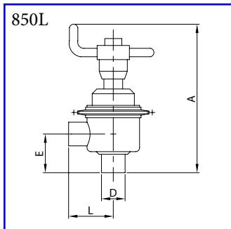
Manual valve 2-ways L - plain ends AISI 304L, AISI 316L
