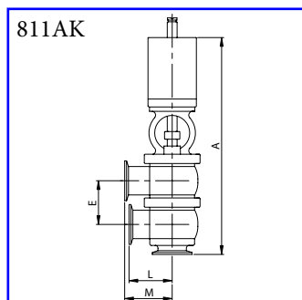
Pneumatic valve 3-A 3-ways LL - CLAMP AISI 316L
