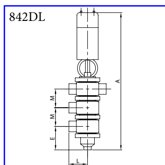
Drainage pneumatic valve 4-ways TLL - plain ends AISI 316L
