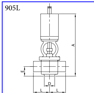
Pneumatic valve 3-A 3-ways T - plain ends AISI 304L, AISI 316L
