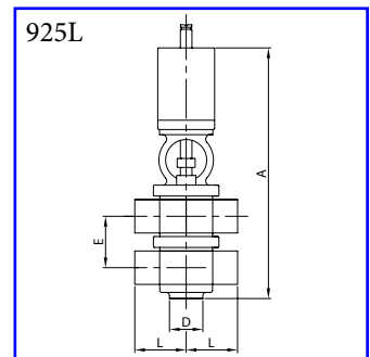
Pneumatic valve 3-A 5-ways TT - plain ends AISI 304L, AISI 316L
