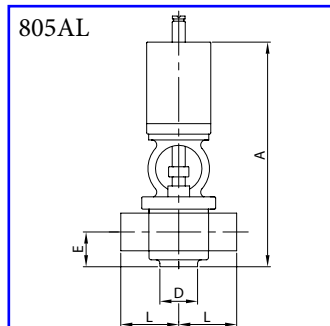
Pneumatic valve 3-A 3-ways T - plain ends AISI 316L
