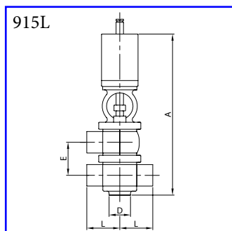
Pneumatic valve 3-A 4-ways LT - plain ends AISI 304L, AISI 316LL
