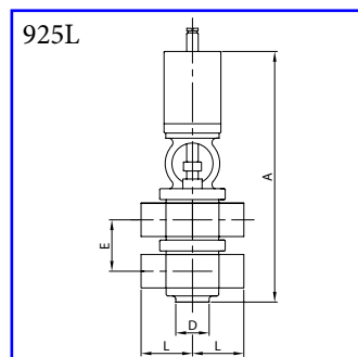
Pneumatic valve 3-A 5-ways TT - plain ends AISI 304L, AISI 316L
