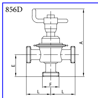
Manual valve 3-ways T - male ends AISI 304L, AISI 316L
