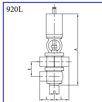
Pneumatic valve 3-A 4-ways TL - plain ends AISI 304L, AISI 316L
