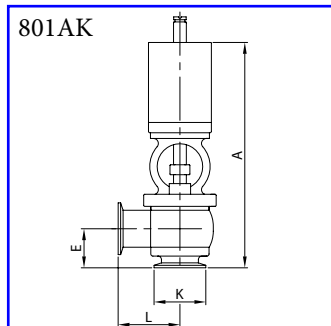
Pneumatic valve 3-A 2-ways L - CLAMP AISI 316L
