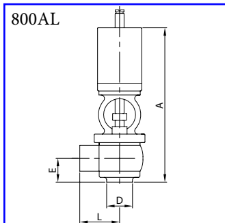
Pneumatic valve 3-A 2-ways L - plain ends AISI 316L
