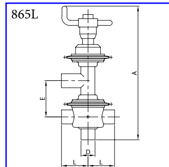
Manual valve 4-ways LT - plain ends AISI 304L, AISI 316L
