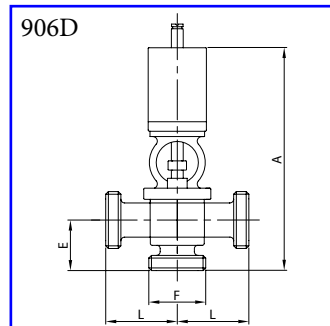
Pneumatic valve 3-A 3-ways T - male ends AISI 304L, AISI 316L
