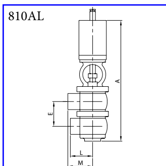
Pneumatic valve 3-A 3-ways LL - plain ends AISI 316L
