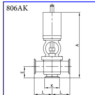
Pneumatic valve 3-A 3-ways T - CLAMP AISI 316L
