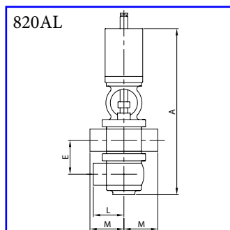
Pneumatic valve 3-A 4-ways TL - plain ends AISI 316L
