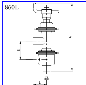
Manual valve 3-ways LL - plain ends AISI 304L, AISI 316L
