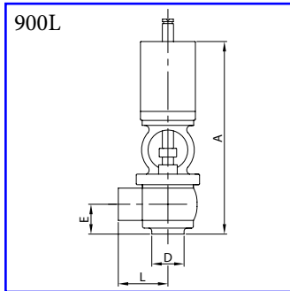
Pneumatic valve 3-A 2-ways L - plain ends AISI 304L, AISI 316L
