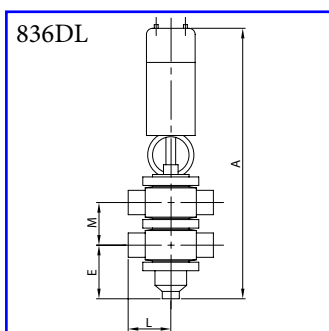
Drainage pneumatic valve 4-ways TT - plain ends AISI 316L
