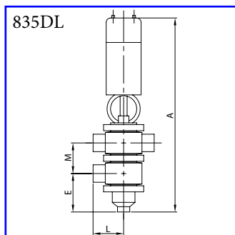
Drainage pneumatic valve 3-ways TL - plain ends AISI 316L
