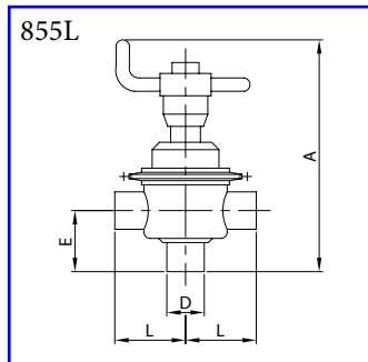
Manual valve 3-ways T - plain ends AISI 304L, AISI 316L
