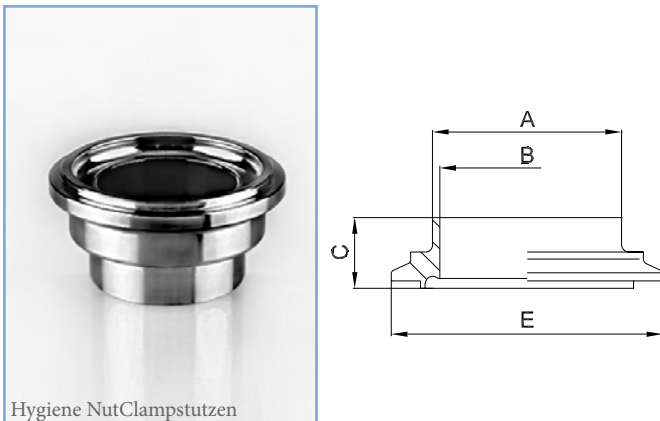
Hygienic Clamp with groove DIN 11853-3:
