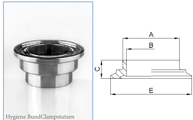
Hygienic Clamp with collar DIN 11853-3:
