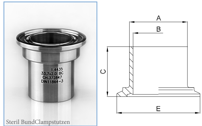
Aseptic Clamp with collar DIN 11864-3-A:
