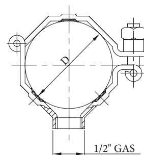
Octagonal pipe hanger with thread
