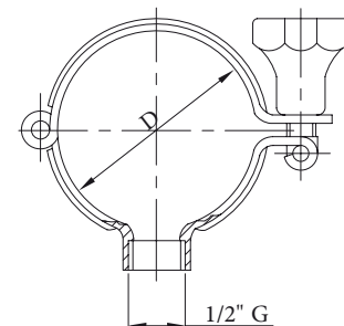
Hinged pipe hanger with thread G
