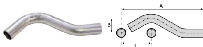
INOX PRESS - Bridge M (press) / M (press)
