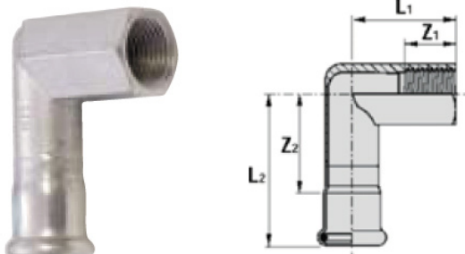
INOX PRESS - 90° Elbow F (press) / female thread BSP
