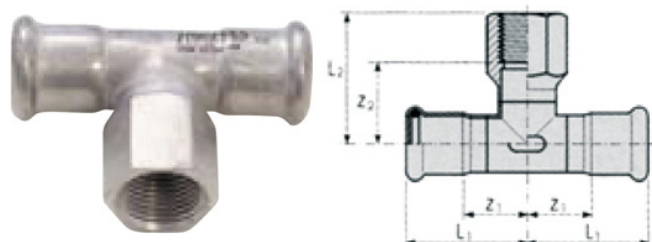
INOX PRESS T-piece adaptor F (press) / F (BSP) / F (press)
