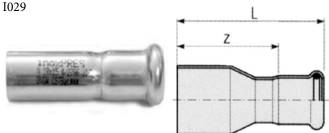
INOX PRESS - Reducer M/F
