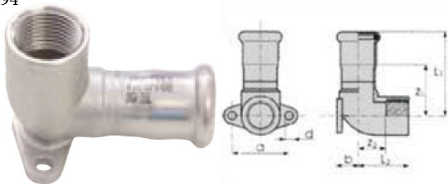
INOX PRESS - 90° Elbow F (press) / female thread BSP with wall plate
