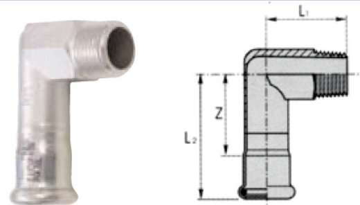
INOX PRESS - 90° Elbow F (press) / male thread BSP
