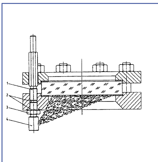
Spraying unit of the series SVS built into circular sightglass to DIN 28120
