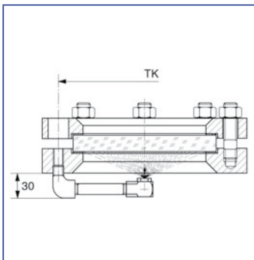
Spraying unit, built into circular sightglass to DIN 28120.
