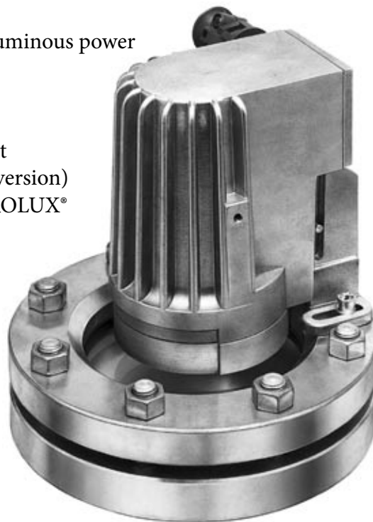
Type PEL 50 deHSch, EEx de IIC T4, Ex II 2 G + D, 230 V, 50 W, mounted on circular sightglass to DIN 28120, DN 125, PN 10, in 2 port version.
