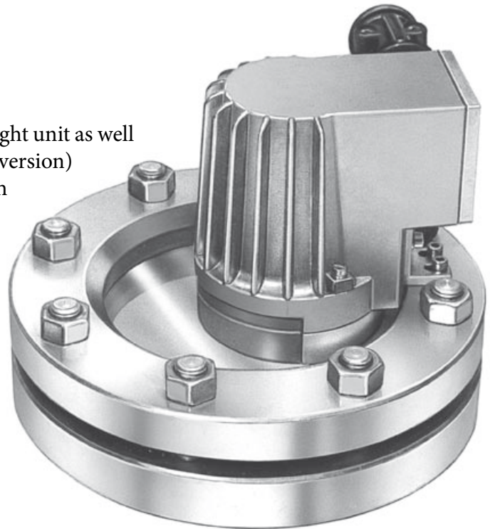
Type KEL 20 deH W, EEx de IIC T4, Ex II 2 G + D, 230 V, 20 W, mounted on circular sightglass to DIN 28120, DN 125, PN 10, in 1 port version.
